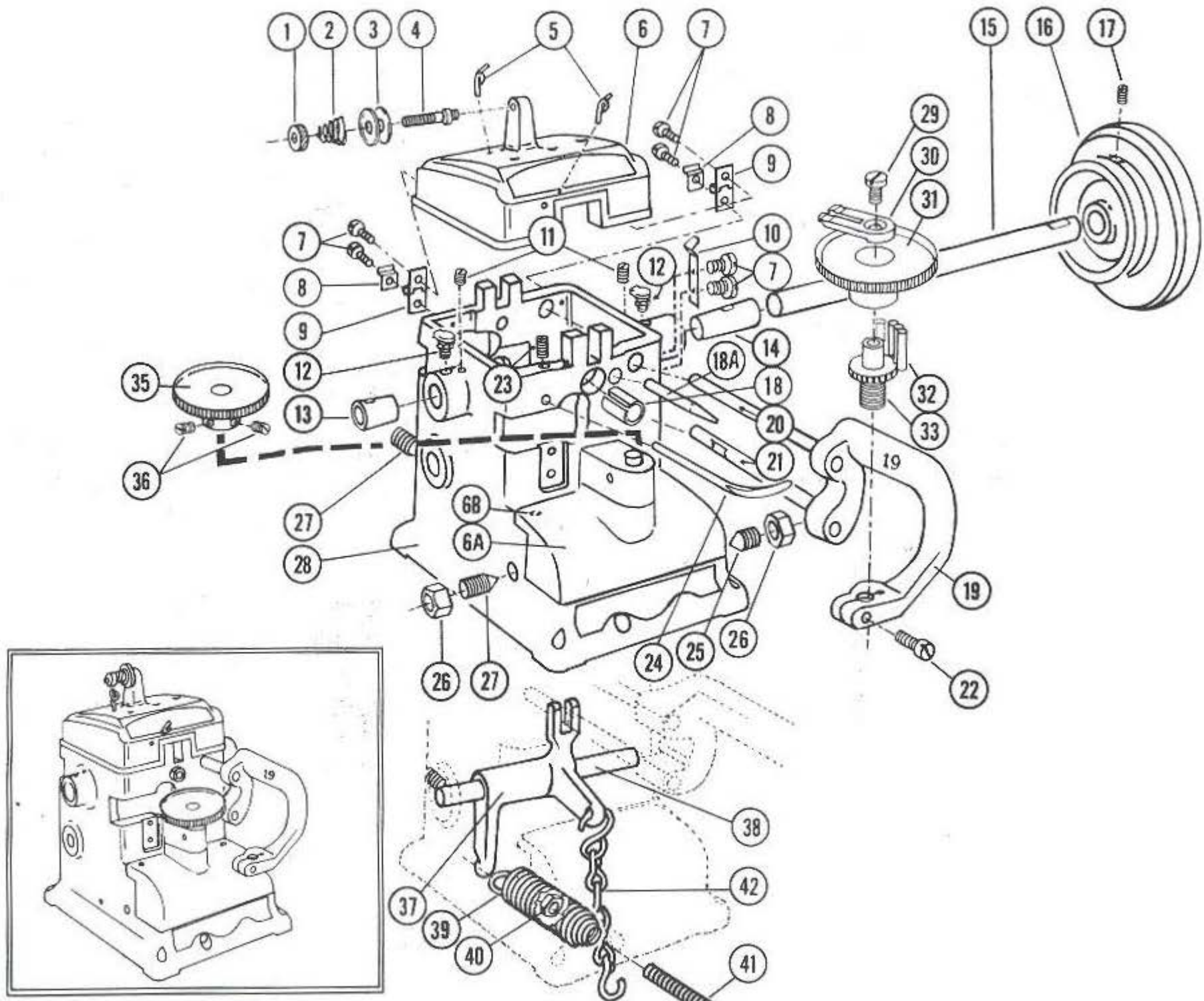
ILLUSTRATION IN BOX SHOWS ARM AND WHEEL ATTACHED TO MAIN FRAME
